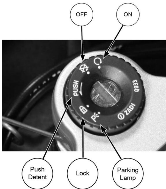
Figure 5. Ignition Switch
